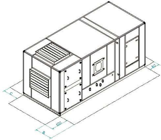
Air Washer
