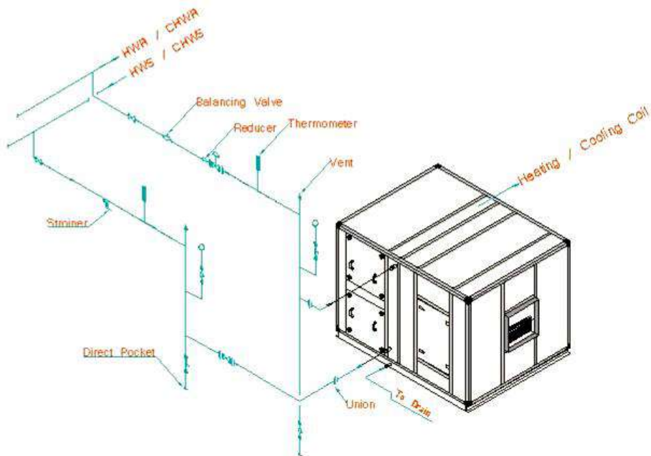
Suggested Coil Connection Details for Heating and Cooling Coils
