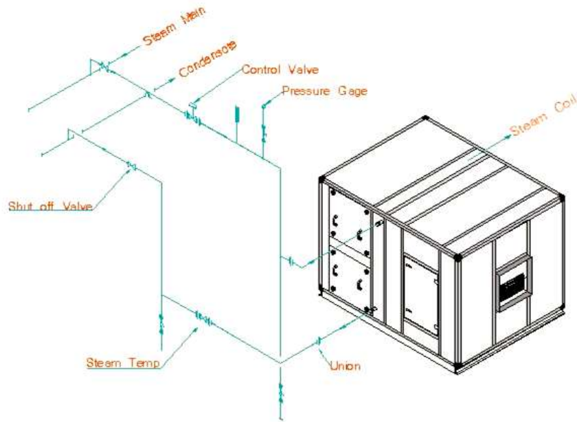
Suggested Coil Connection Details for Steam Coils
